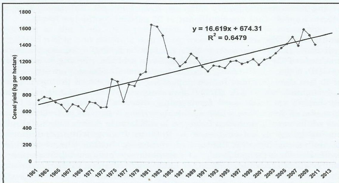
Figure 1: Cereal yield in Nigeria over the years
