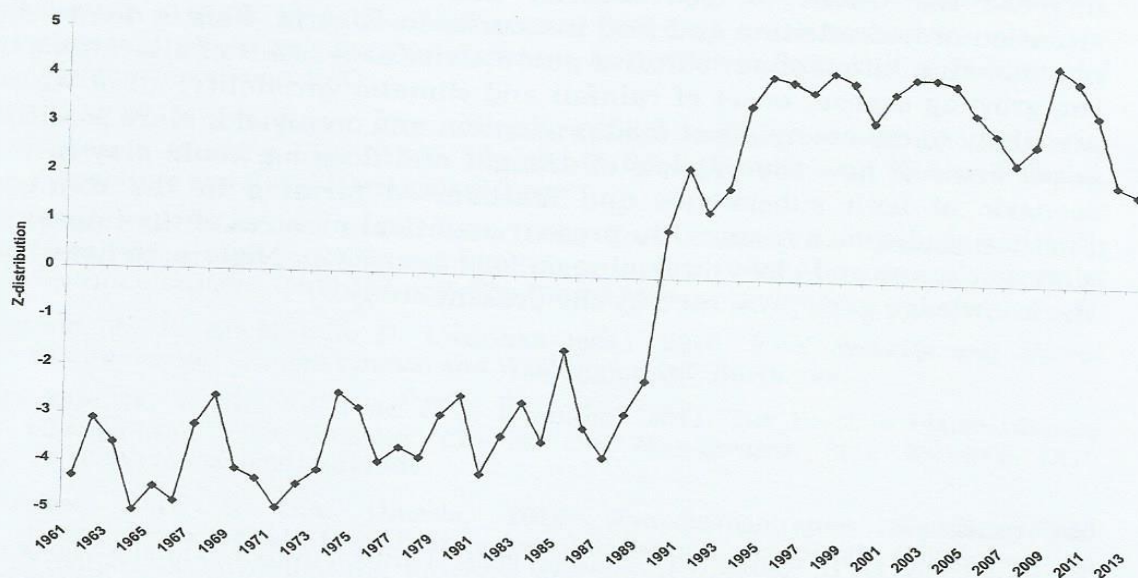
Figure 3: Z-distribution array of the impact of climatic variability on food security
