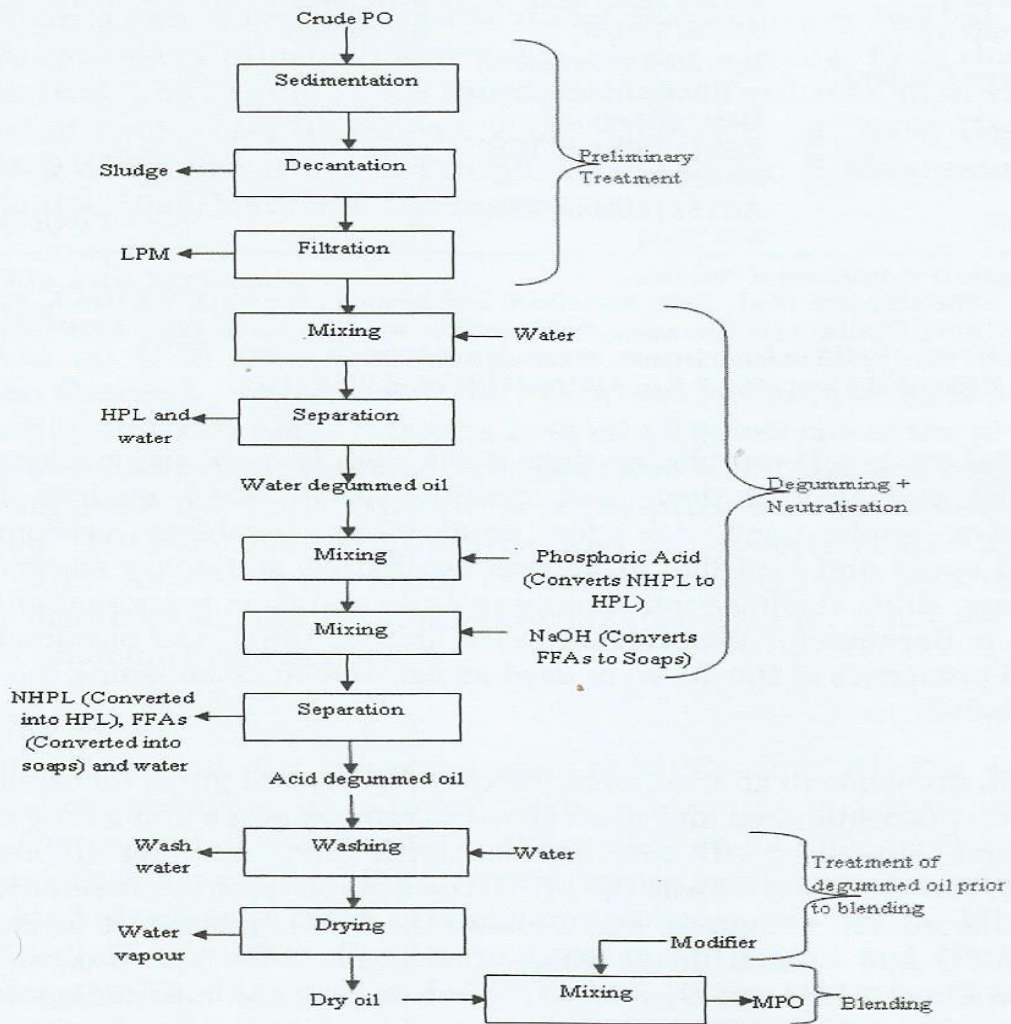
Figure 2: Flow Diagram for Producing MPO
