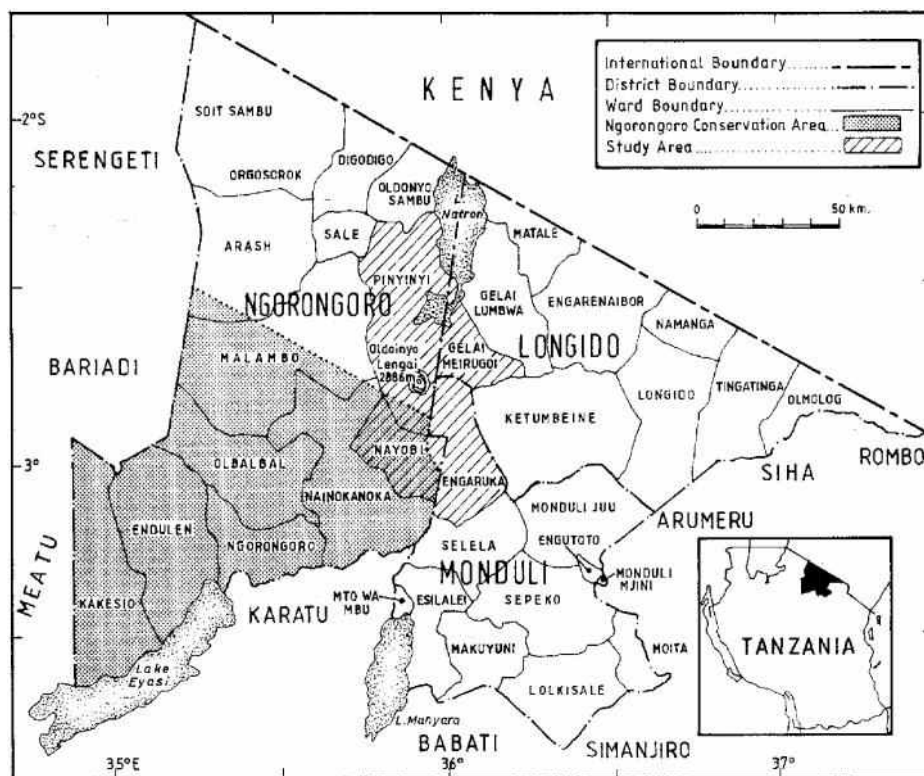
Figure 1.1: Location of Oldoinyo Lengai and its vicinity
